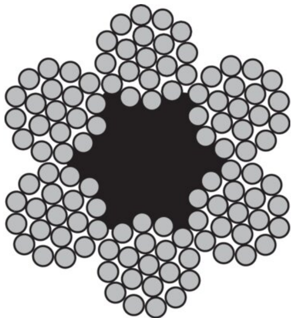
Stropen-kabel
